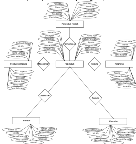
Gambar 11. ERD (Entity Relationship Diagram)
