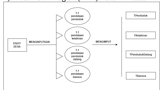
Gambar 8. DFD Level 1 proses 1
