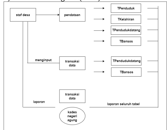
Gambar 7. DFD Level 0 Proses 1
