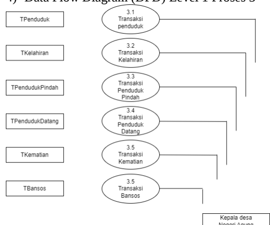
Gambar 10. DFD Level 1 Proses 3
