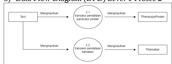
Gambar 9. DFD Level 1 Proses 2
