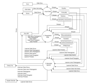
Gambar 2. Data Flow Diagram (DFD) Level 0
