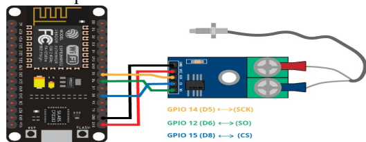
Gambar 1. Tampilan rancangan hardware smart cooker
